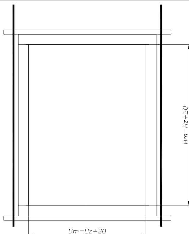
Figure 5. Preparing installation opening in self supporting ducts.
