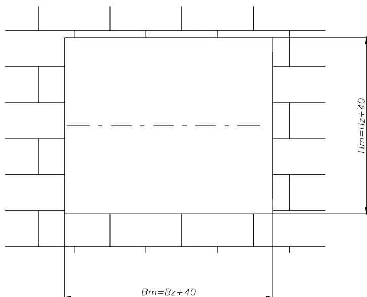
Figure 4. Preparing installation opening in brickwork and concrete walls.
