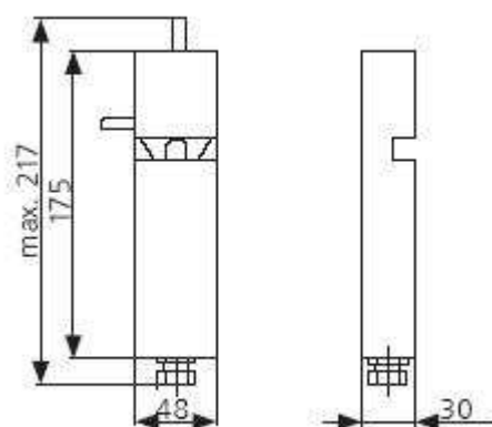
Figure 8. Control release mechanism EM24D.
