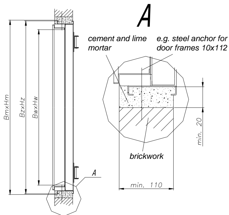
Figure 6. Fire damper mcr-DOR – installation in brickwork and concrete walls.
