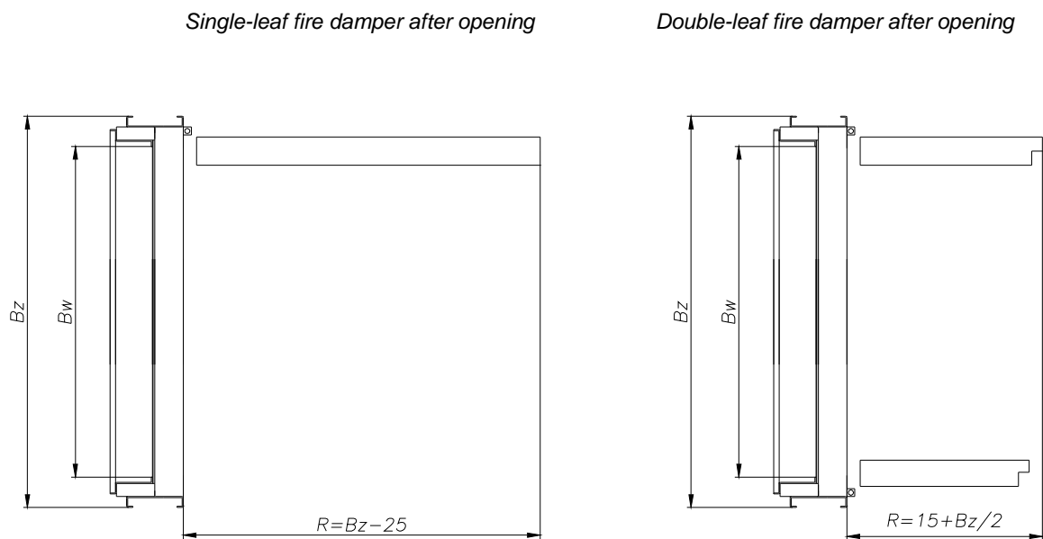
Figure 3. Fire dampers mcr-DOR after opening the baffle
